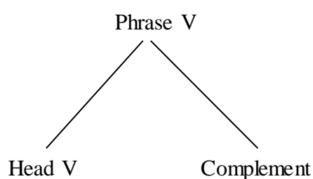
Figure 1. Phrase Structure
